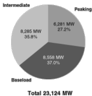
Approximate U.S. Portfolio Net Capacity By Dispatch Level
